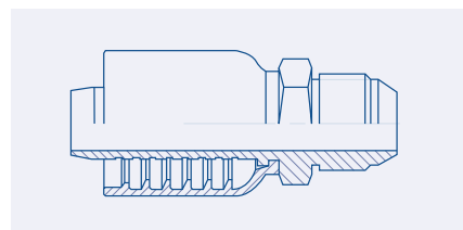
Male SAE 45° Rigid - MX BW23.2S00.
