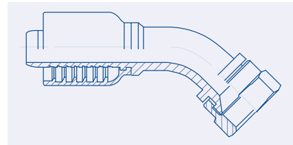
Female JIC 37° Swivel 45° Elbow - FJ45 BW23.4042.
