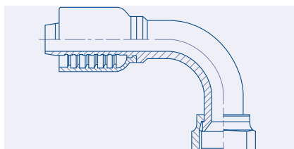
Female SAE 45° Swivel 90° Elbow - FX90 BW23.4S92.
