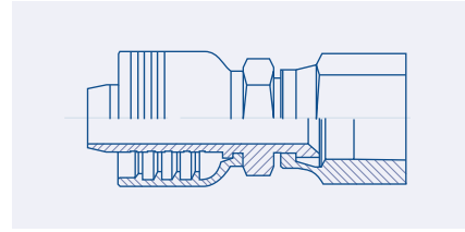
Female JIC 37° Swivel - FJ
