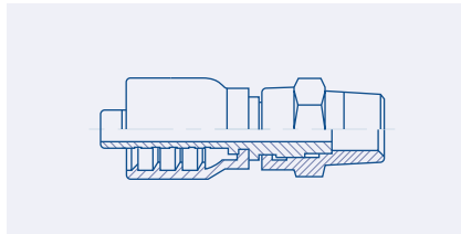
Male NPTF Swivel - MPX BW23.0410.
