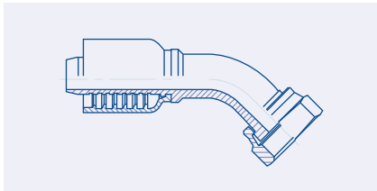
Female ORFS Swivel 45° Elbow - OFT45
