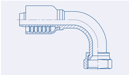
Female JIC 37° Swivel 90° Elbow - FJ90 BW23.4092.
