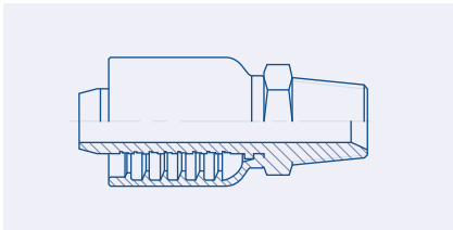
Male NPTF Pipe Rigid - MP BW23.0400.
