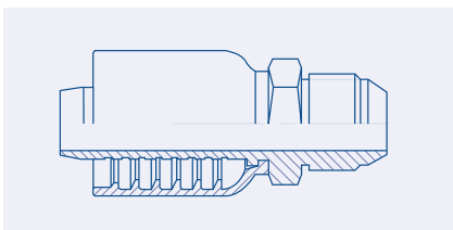
Male JIC 37° Rigid - MJ BW23.2000.
