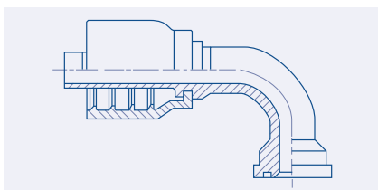
90° Elbow SAE 3000 PSI Code 61 Flange - PA90
