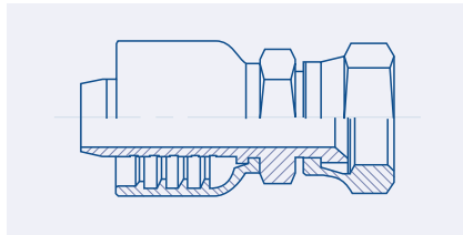
Female JIC 37° Swivel - FJ BW23.4H12.
