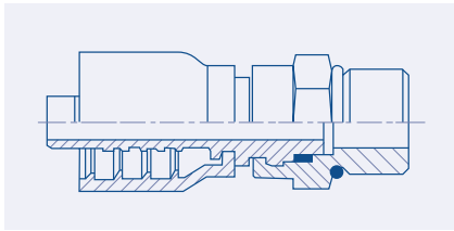
SAE Straight Swivel O-ring Boss Male - RAX
