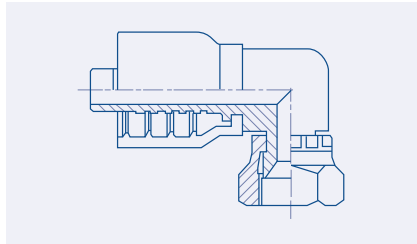
Female JIC 37° Swivel 90° Short Elbow - FJ90S BW23.4082.
