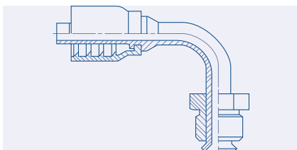
SAE Inverted 45° Flare 90° Elbow Male - MSAE 90
