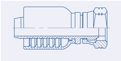
Female NPSM Pipe Swivel - FPX BW23.3010.
