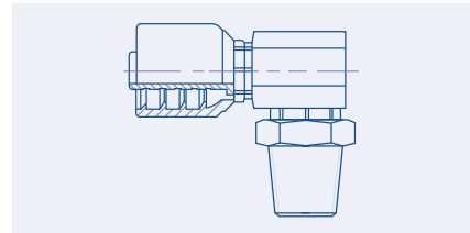
Male NPTF Swivel 90° Elbow - MPX90 BW23.0490.
