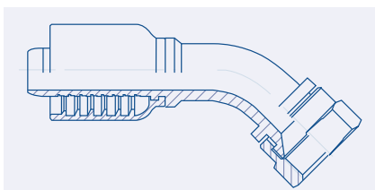
Female SAE 45° Swivel 45° Elbow - FX45 BW23.4S42.
