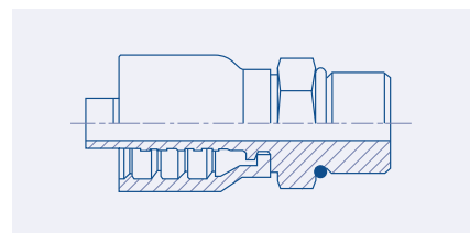
SAE Straight O-ring Boss Male - RA BW23.2010.
