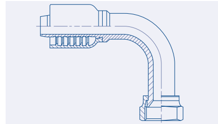
Female JIC 37° Swivel 90° Long Elbow - FJ90L BW23.4092L.
