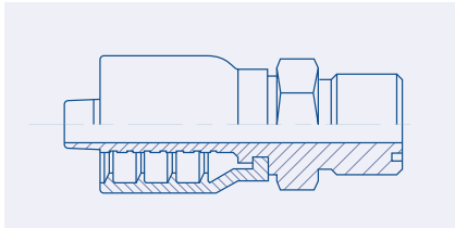
Male ORFS - OFTM
