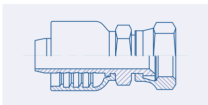
Female SAE 45° Swivel - FX BW23.SH12.
