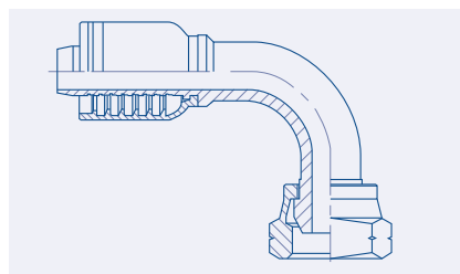
BSP 60° Swivel 90° Elbow Female - BSPXF90 BF21.3092. pag. 58
