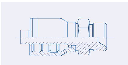
BSP 60° Male - BSPM BF21.0100. pag. 59
