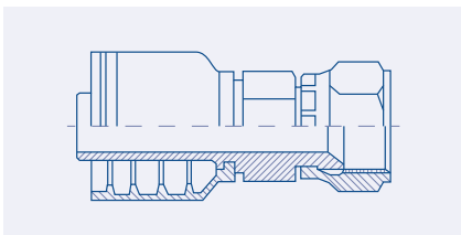
JIS 30° Female Swivel - FX-KOMA BF21.5911. pag. 53
