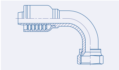
Female JIC 37° Swivel 90° Elbow - FJ90
