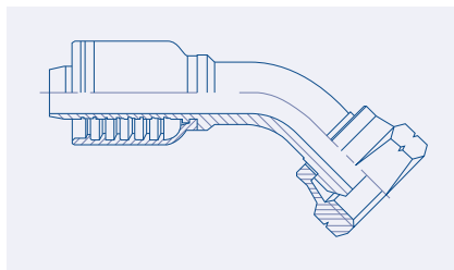
BSP 60° Swivel 45° Elbow Female - BSPXF45 BF21.3042. pag. 57
