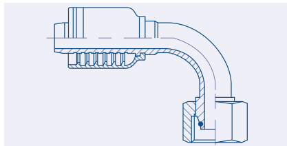
Heavy 24° Metric 90° Elbow Female - DHF90 BF21.5193. pag. 51
