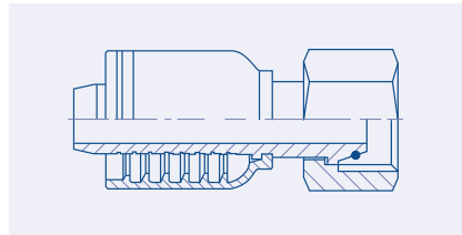
Heavy 24° Metric Female - DHF BF21.5113. pag. 49
