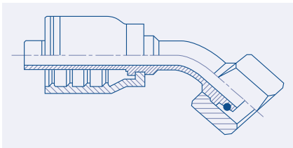
Heavy 24° Metric 45° Elbow Female - DHF45 BF21.5143. pag. 50
