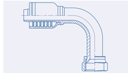
Female JIC 37° Swivel 90° Long Elbow - FJ90L
