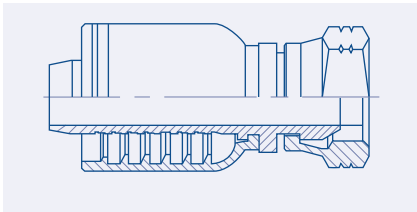
Female NPSM Pipe Swivel - FPX
