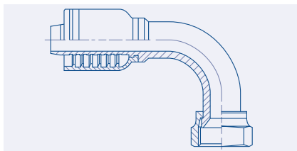
Female JIS 30° Swivel 90° Elbow - FX-KOMA90 BF21.5991. pag. 54
