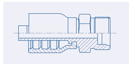
Heavy 24° Metric Male - DHM
